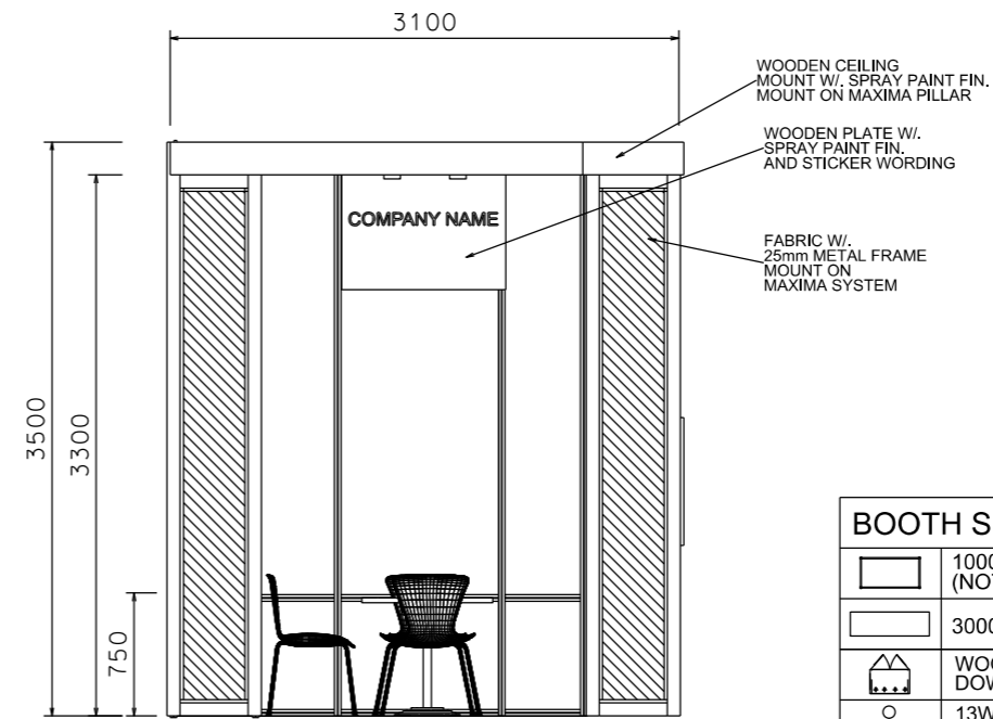
PERSPECTIVE
