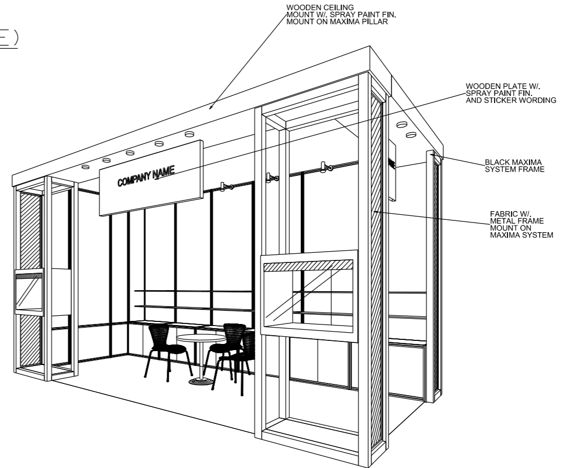
PERSPECTIVE
