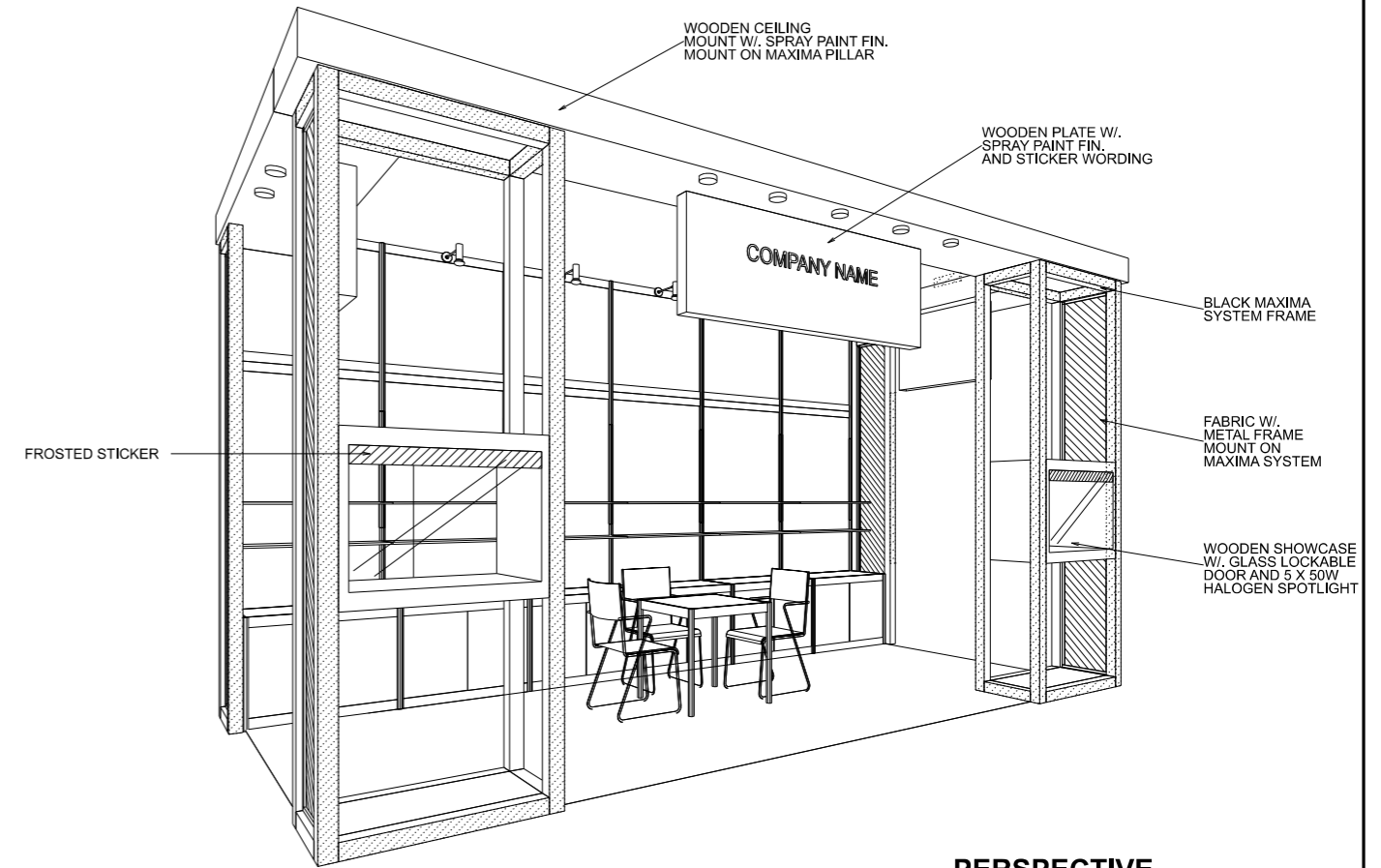
PERSPECTIVE
