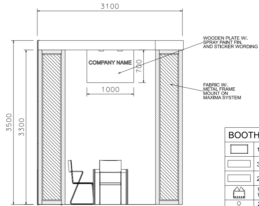
RIGHT SIDE
