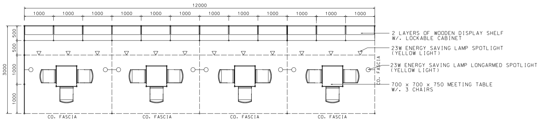
PLAN
